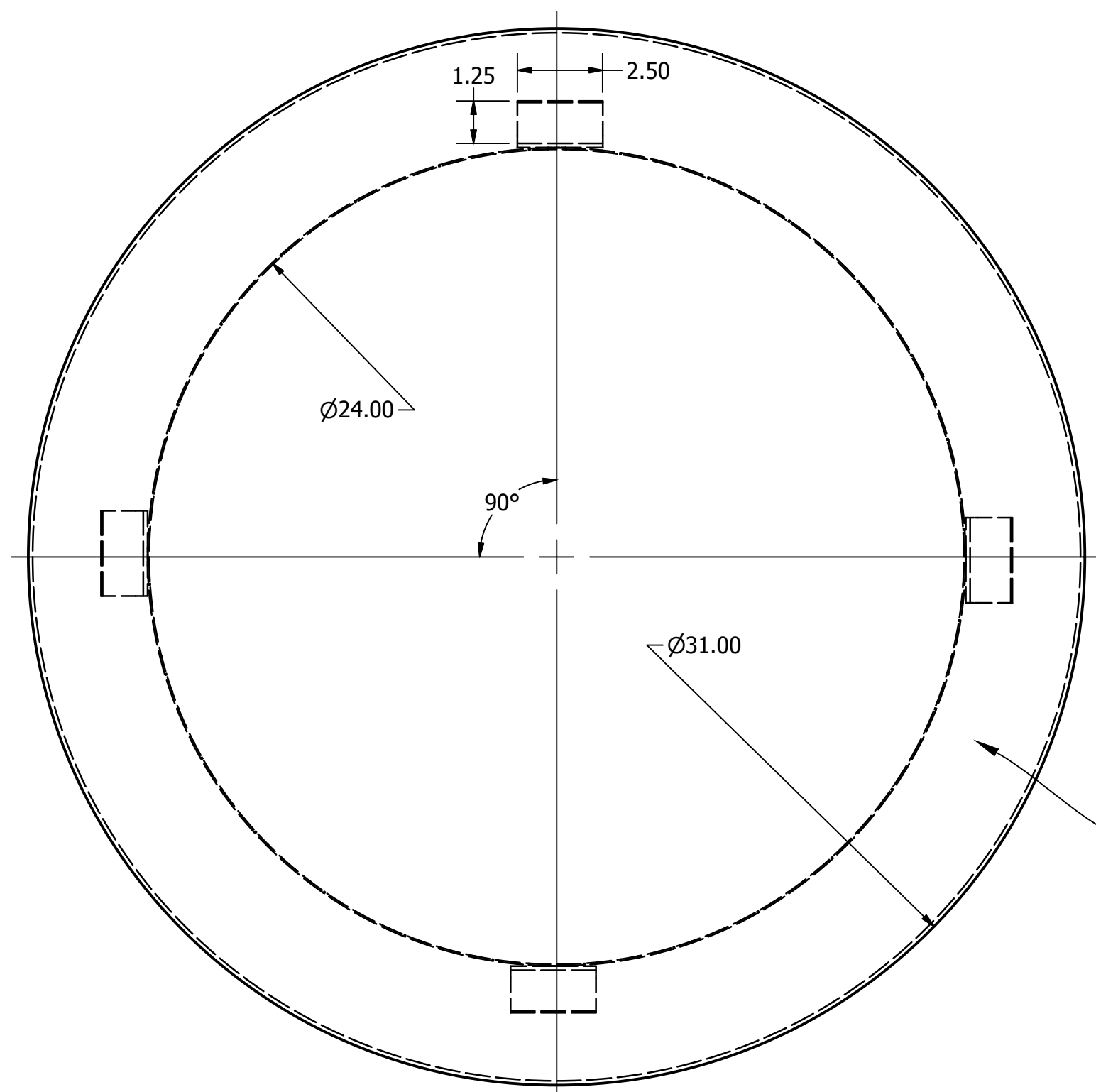
TOP SCALE 1 / 4
