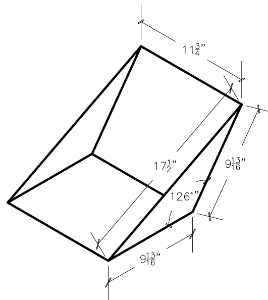
HOPPER DETAIL
