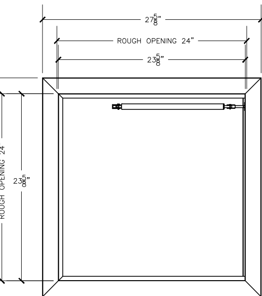
REAR VIEW
