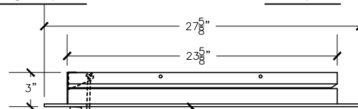
RIGHT VIEW
