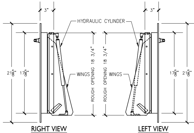
RIGHT VIEW RUBBER BAFFLE NOT SHOWN
