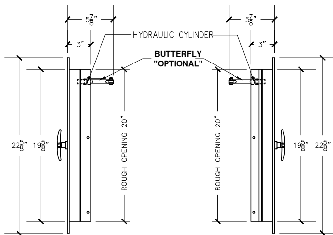
RIGHT VIEW
