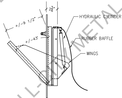
TRASH DOOR AT OPENED POSITION
