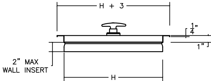
LINEN SIDE ELEVATION
