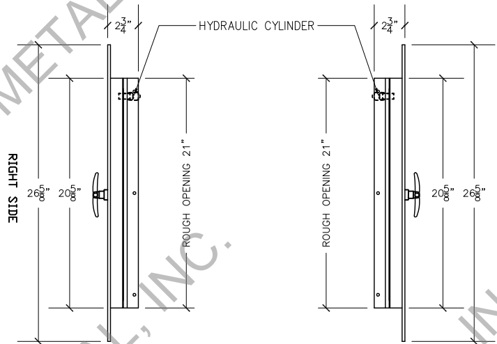
RIGHT VIEW
