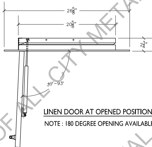
RIGHT VIEW
