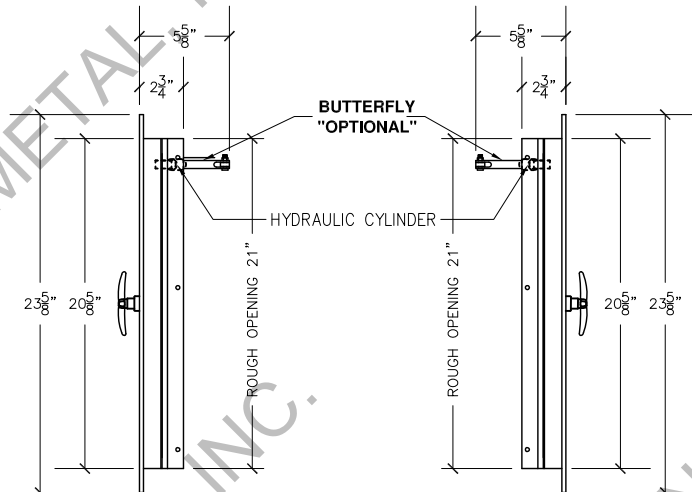
RIGHT VIEW
