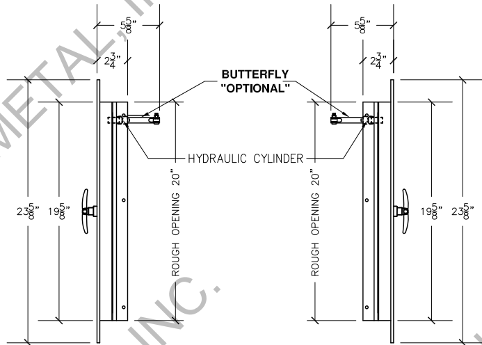
RIGHT VIEW
