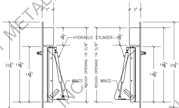
RIGHT VIEW
