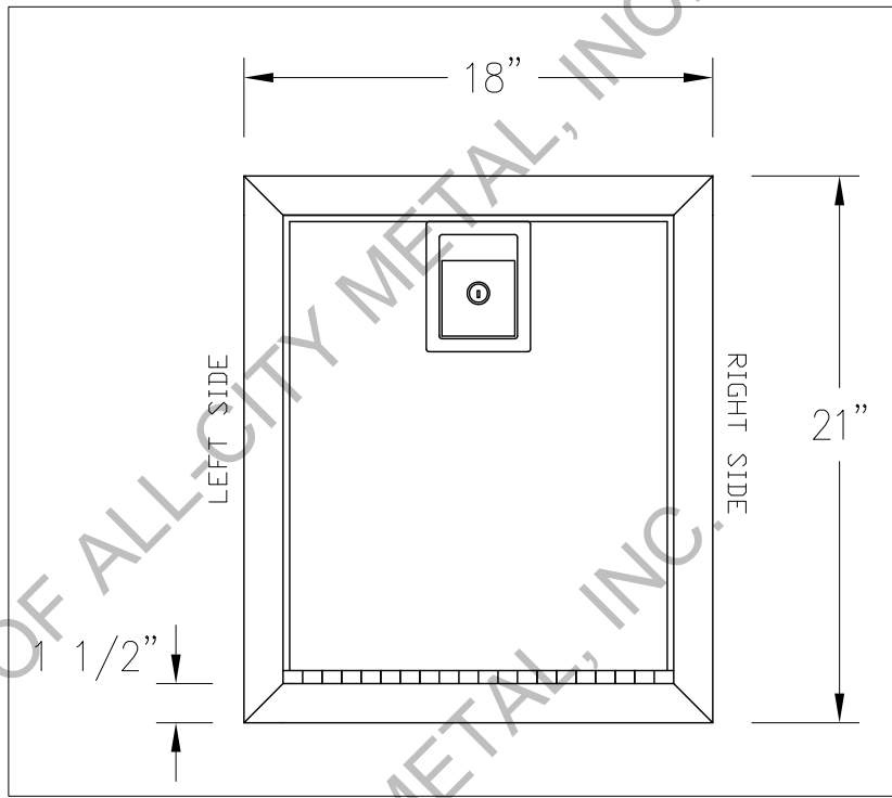
CHUTE DOOR/ FLUSH MOUNTED HANDLE
