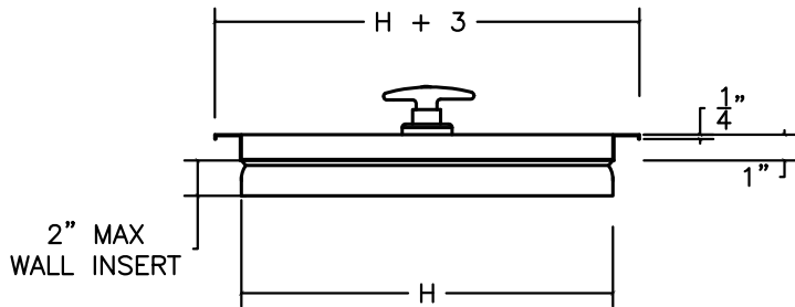
ACCESS DOOR SIDE ELEVATION
